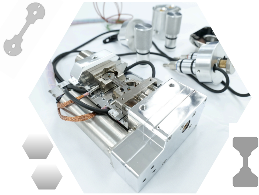
Micromachines for thermomechanical tests
